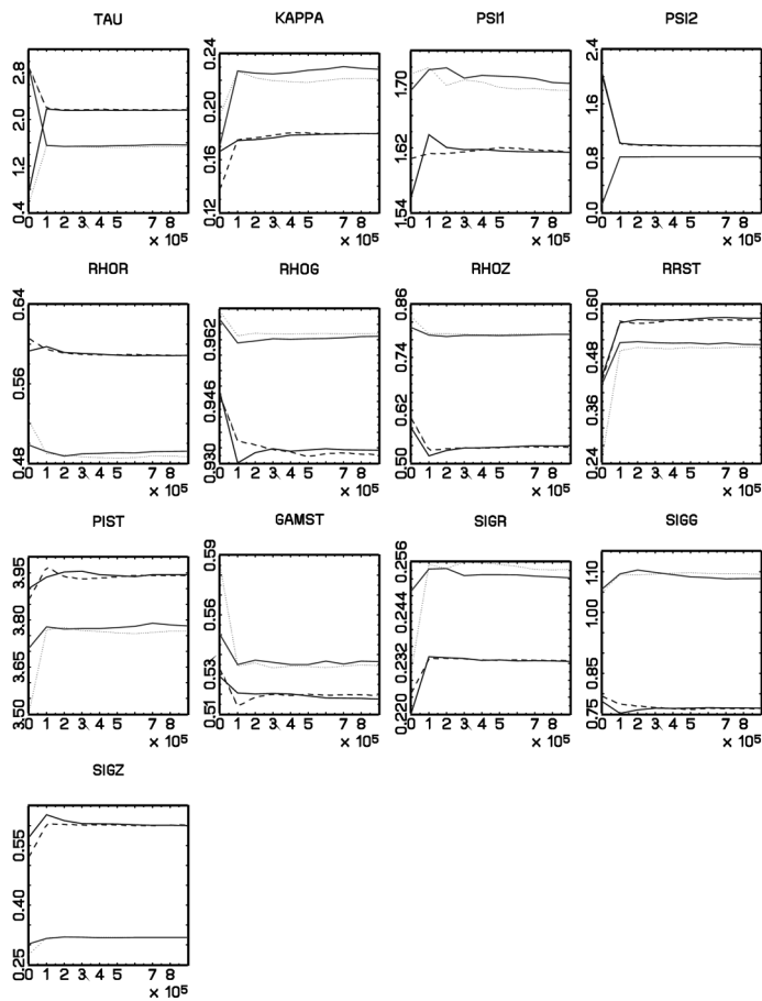
FIGURE 6 Recursive means from multiple chains – Model \mathcal{M}_2(L) , Data \mathcal{D}_1(L) . Each line corresponds to recursive means (as a function of the number of draws) calculated from one of the four Markov chains generated by the metropolis algorithm.
